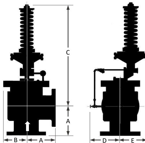
Angle Body Installation Dimensions
