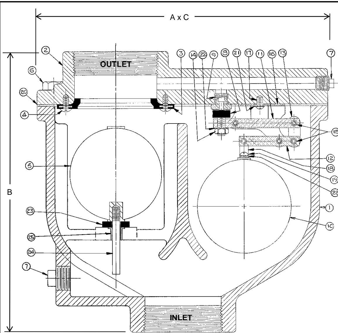
FIGURE 945 COMBINATION AIR VALVES ARE MANUFACTURED AND TESTED IN ACCORDANCE WITH AWWA C512
