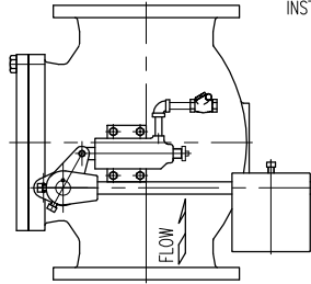
VERTICAL INSTALLATION
