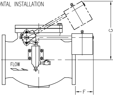
HORIZONTAL INSTALLATION
