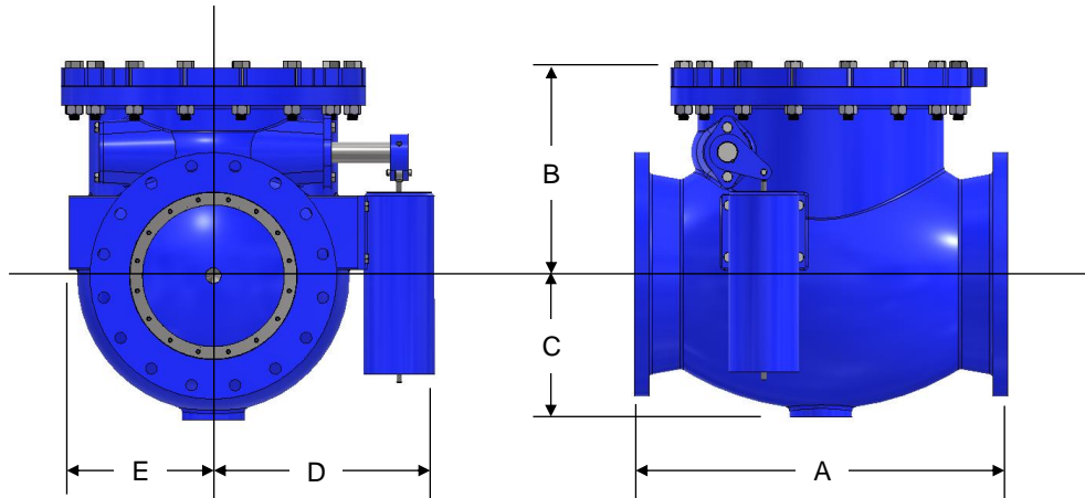
Installation Dimensions
