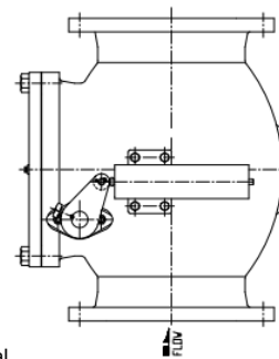
Vertical Installation
