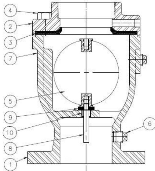
Figure 2 Flanged Inlet
