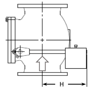
VERTICAL INSTALLATION
