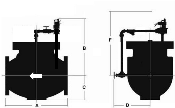
Globe Body Installation Dimensions
