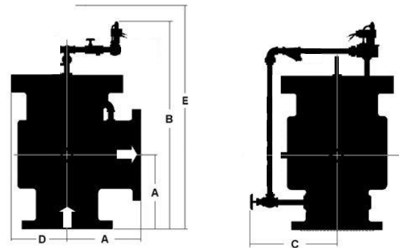
Angle Body Installation Dimensions
